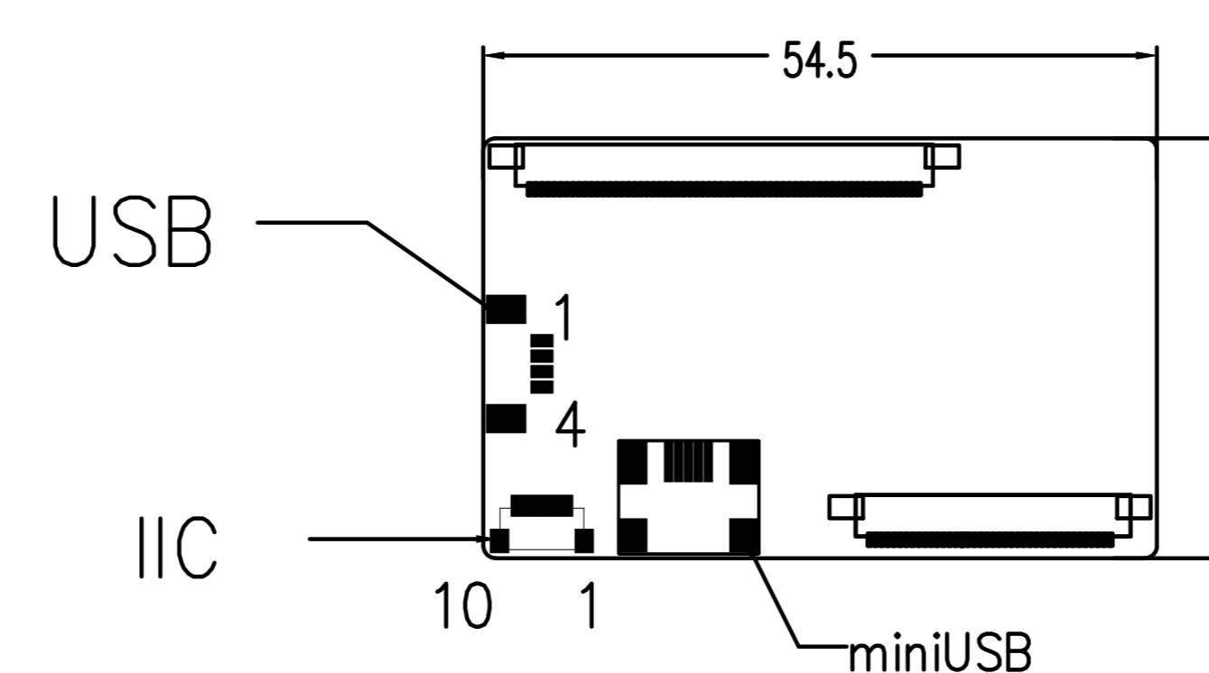
PCB Board SCALE 3:1
